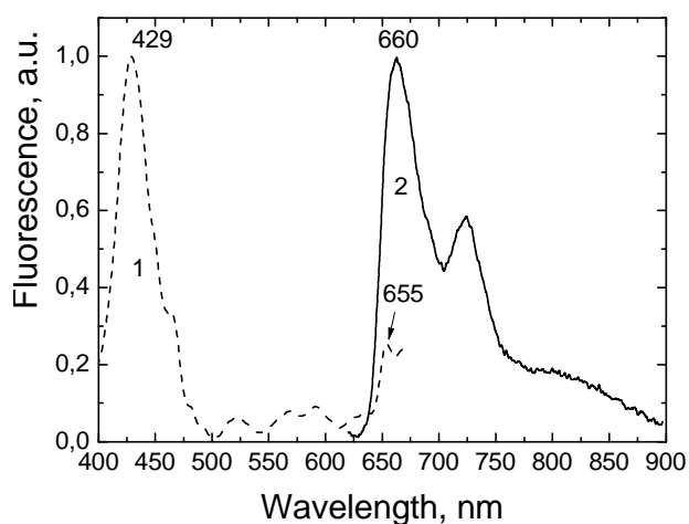
Figure 6. Fluorescence excitation (1, \lambda_{\text{reg}}=720 nm) and fluorescence (2, \lambda_{\text{exc}}=420 nm) spectra of tetra( p -aminophenyl)porphyrin (TAPP) attached to polypropylene film 6B, treated in afterglow of O_2 -plasma (295 K).
